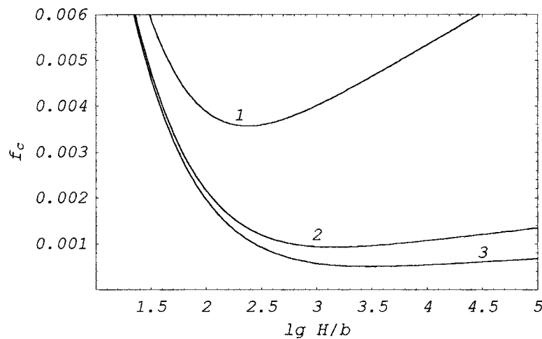
Figure 6. The dependences of critical misfit parameter f_c on \log H/b . Curves 1, 2 and 3 correspond to substrate radius R_1 = 100b, 500b, 1000b , respectively.
