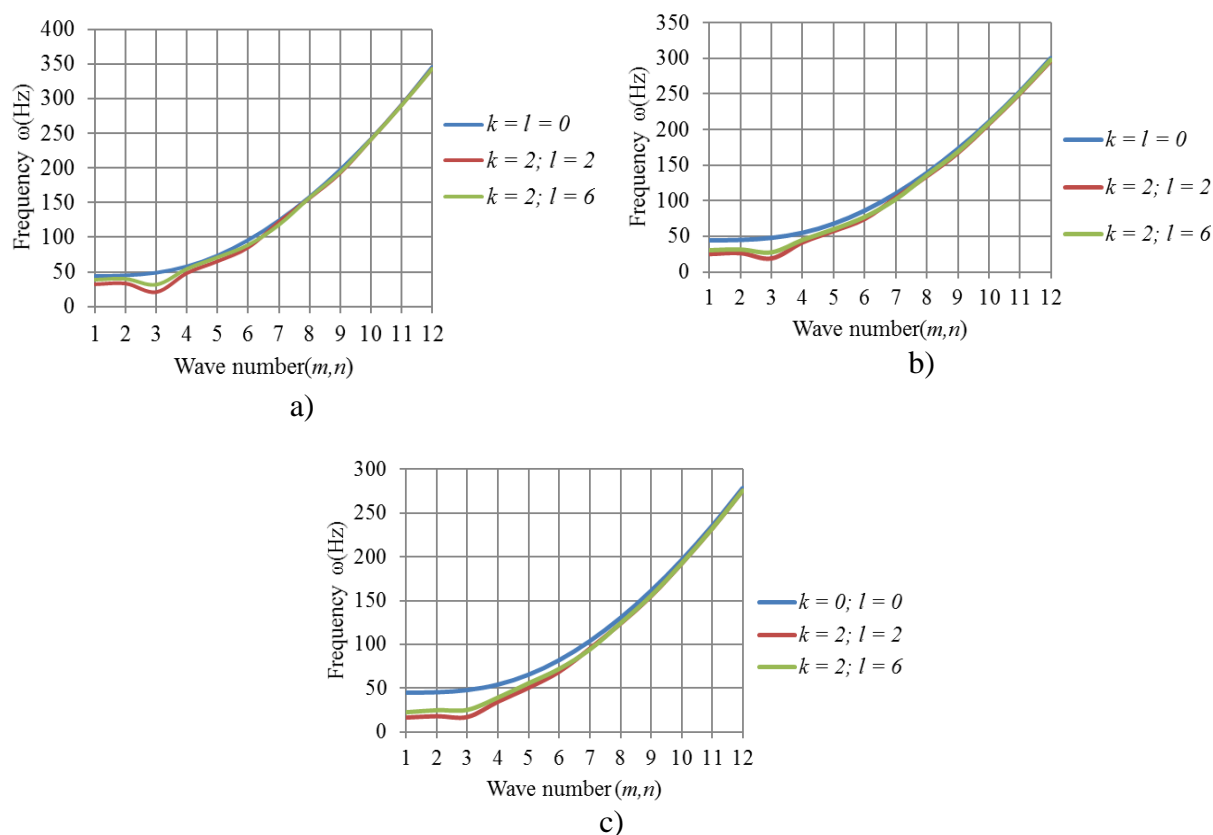
Fig. 1. Dependency graphs of free oscillations on various parameters a – shell 8x12 m; b – shell 8x16 m; c – shell 8x20 m.
