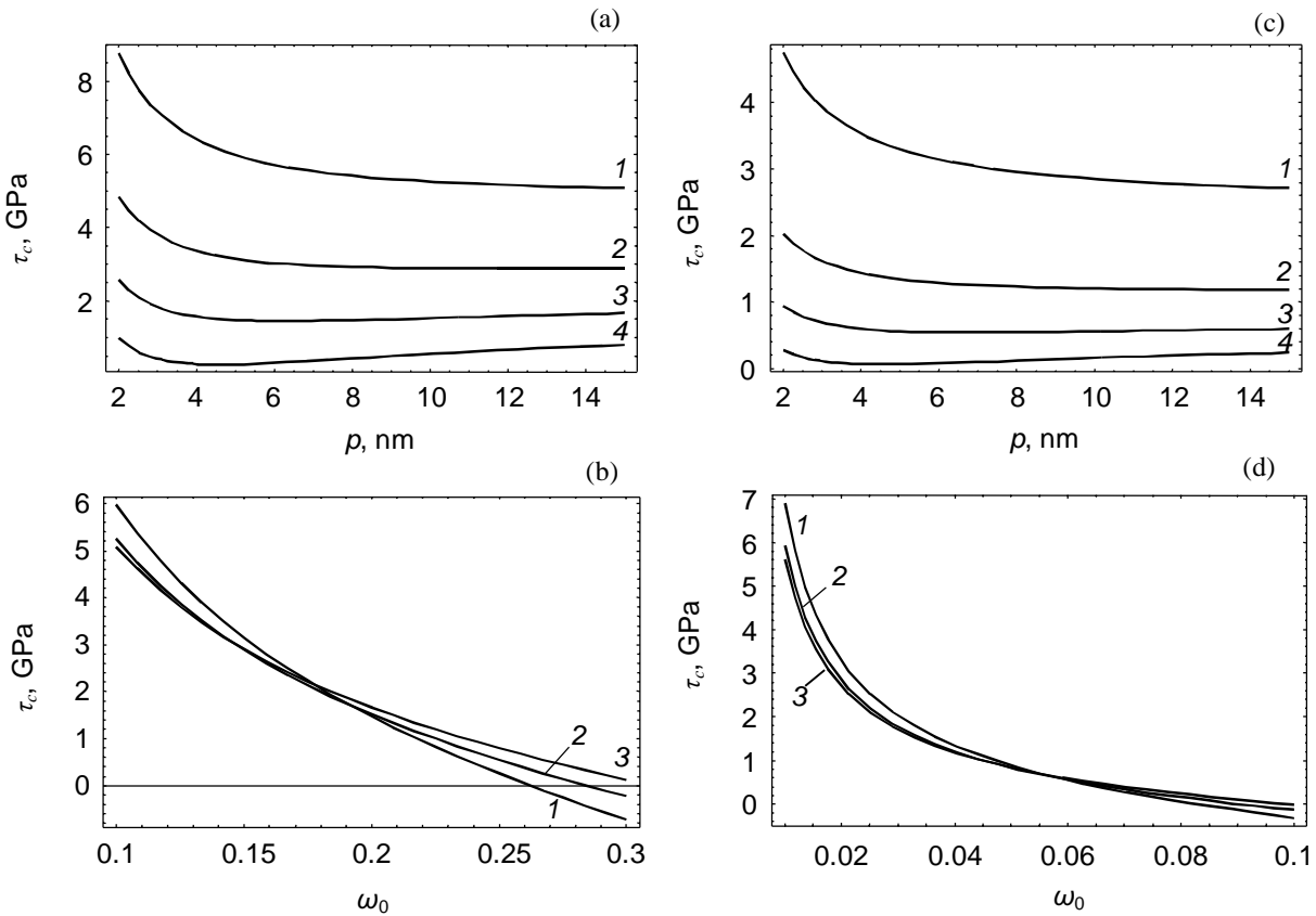
Fig. 9. The dependence of the critical shear stress \tau_c in nanocrystalline \alpha - \text{Al}_2\text{O}_3 (a) on the size p of the disclination dipole AB in the situation with the nucleation of a nanograin with all general GBs (curves 1, 2, 3 and 4 correspond to \omega_0 = 0.1, 0.15, 0.2, and 0.25 , respectively); (b) on parameter \omega_0 in the situation with the nucleation of a nanograin with all general GBs (curves 1, 2, and 3 correspond to p = 5, 10, and 15 nm, respectively); (c) on the size p of the disclination dipole AB in the situation with the nucleation of a nanograin having two general and two special GBs (curves 1, 2, 3, and 4 correspond to \omega_0 = 0.02, 0.04, 0.06, and 0.08 , respectively); (d) on parameter \omega_0 in the situation with the nucleation of a nanograin having two general and two special GBs (curves 1, 2, and 3 correspond to p = 5, 10, and 15 nm, respectively).
