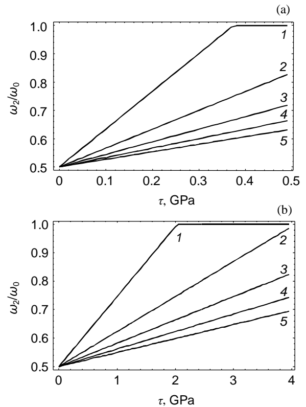
Fig. 10. Dependence of the ratio \omega_2/\omega_0 (at which the nanograin nucleation is most favourable) on the external stress t . Curves 1, 2, 3, 4, and 5 correspond to values of \omega_0 = 0.1, 0.2, 0.3, 0.4, and 0.5 , respectively. They are presented in the case of p = 5 nm.
