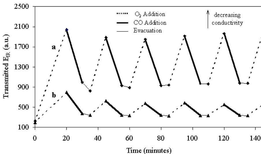
Fig. 2. Variations of the infrared energy ( E_{IR} ) transmitted by the SnO 2 nanoparticles versus gas exposures: a) at 300 °C; b) at 150 °C.
