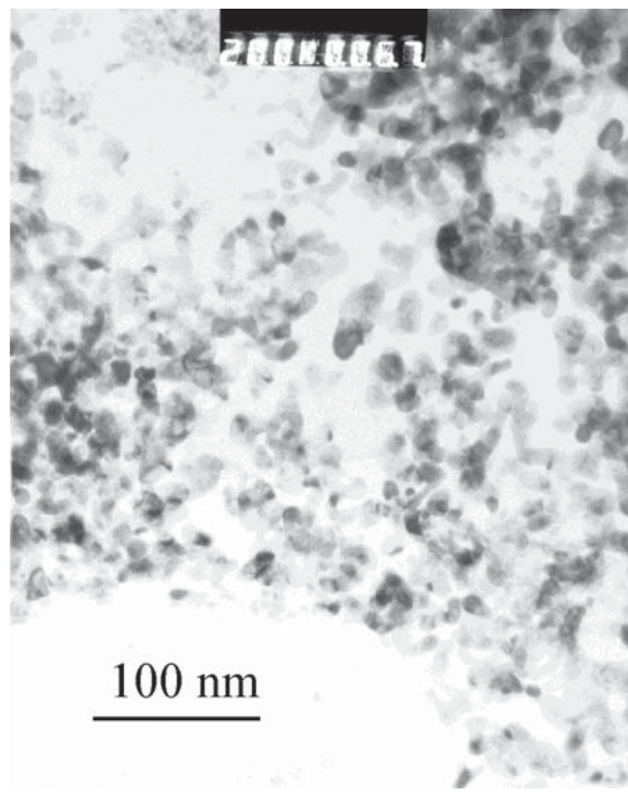
Fig. 3. TEM micrograph of sample M2 showing the morphology of the individual particles in a Pt cluster.
