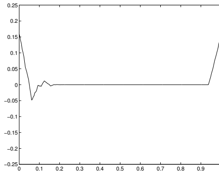
Figure 1: Periodic wavelet
