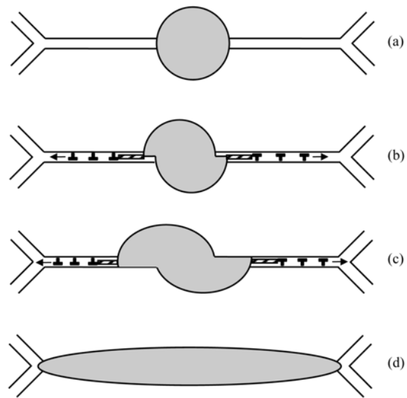
Fig. 5. Elongation of nanovoid due to numerous events of emission of grain boundary dislocations by the new mechanism in deformed polysilicon.
